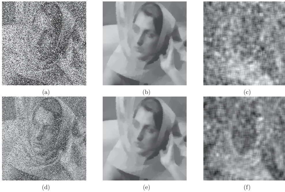
Figure 1. Local expected absolute estimator, salt and pepper noise, (a) noisy image, (b) reconstructed image for too small regularization parameter \lambda , (c) LEAVE^{11} . Random-valued impulse noise, (d) noisy image, (e) reconstructed image for too small regularization parameter \lambda , (f) LEAVE^{11} .
