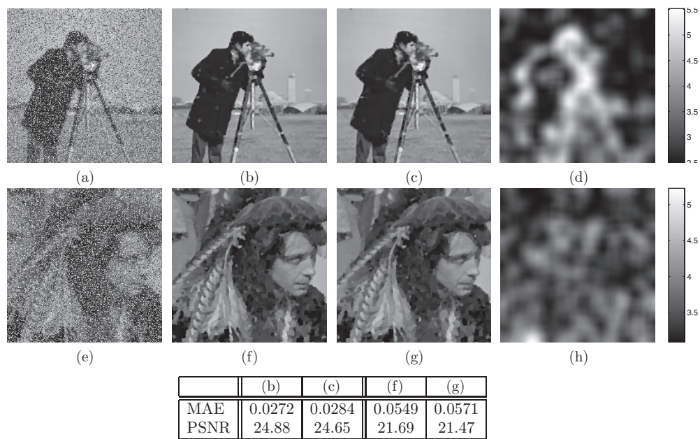
Figure 8. Cameraman : (a) image with blur and random-valued impulse noise r = 0.4 , (b) denoising and deblurring with the L^1 -TV model, \lambda = 3 , (c) denoising and deblurring with the present method, (d) Resulting \lambda . Man : (e) image with blur and random-valued impulse noise r = 0.5 . (f) denoising and deblurring with the L^1 -TV model, \lambda = 3 . (g) denoising and deblurring with the present method and (h) resulting \lambda .
