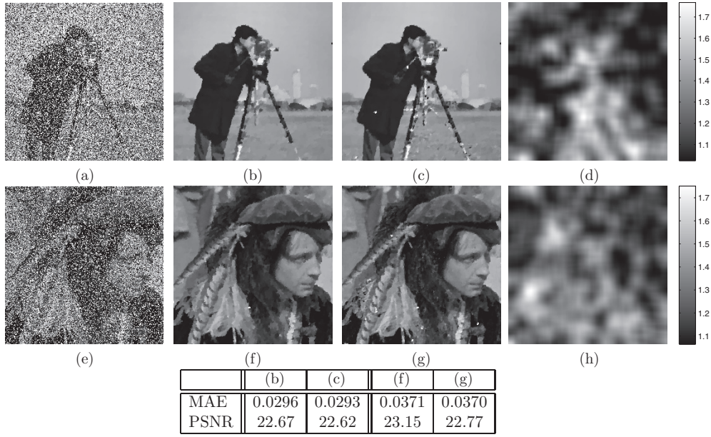
Figure 5. Cameraman : (a) image with salt and pepper noise r = 0.5 , (b) denoising with L^1 -TV model, \lambda = 1.2 , (c) denoising with the present method, (d) resulting \lambda . Man : (e) image with salt-and-pepper noise r = 0.4 , (f) denoising with the L^1 -TV model, \lambda = 1.3 , (g) denoising with the present method and (h) resulting \lambda .
