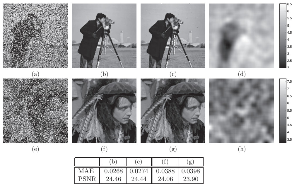
Figure 7. Cameraman : (a) image with blur and salt-and-pepper noise r = 0.5 , (b) denoising and deblurring with the L^1 -TV model, \lambda = 3 , (c) denoising and deblurring with the present method, (d) resulting \lambda . Man : (e) image with blur and salt and pepper noise r = 0.5 , (f) denoising and deblurring with the L^1 -TV model, \lambda = 3 , (g) denoising and deblurring with the present method and (h) resulting \lambda .
